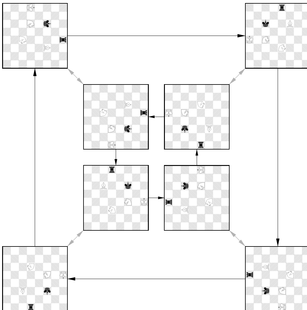
Figure 5. The Cayley graph for \mathfrak{D}_4 . Each node is pictured by showing the effect of its corresponding transformation on a position in \text{♔♕♖♗♘♙♚♛♜♝} ; thus, the chess value of each of these nodes is the same. Black arrows correspond to \tau , and rotate the board counterclockwise 90^\circ . Gray (diagonal) arrows correspond to \mathfrak{f} , and flip the board horizontally. The position shown arose during a game between Anatoly Karpov and Gary Kasparov in Tilburg, October 1991.
